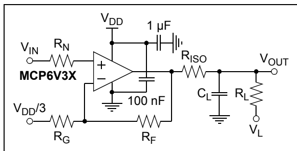
The circuits used for most DC and AC tests are shown in Figure 1-4 and Figure 1-5 . Lay the bypass capacitors out as discussed in Section 4.3.10 “Supply Bypassing and Filtering” . R_N is equal to the parallel combination of R_F and R_G to minimize bias current effects.
