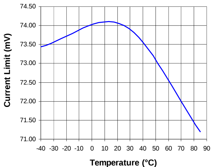
Current Limit vs Temperature
