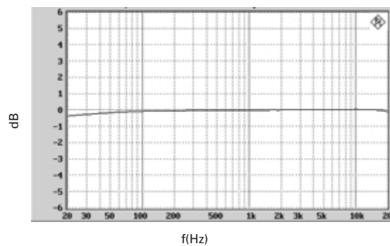
Frequency response (4 load)
