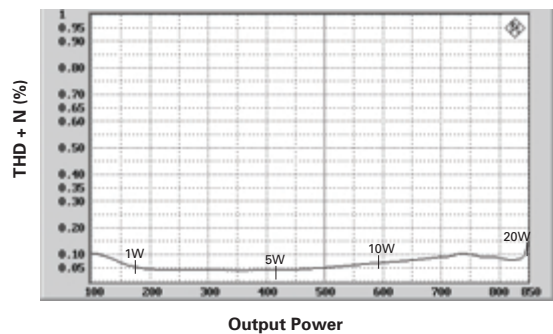
THD v Power into 4 at 1kHz
