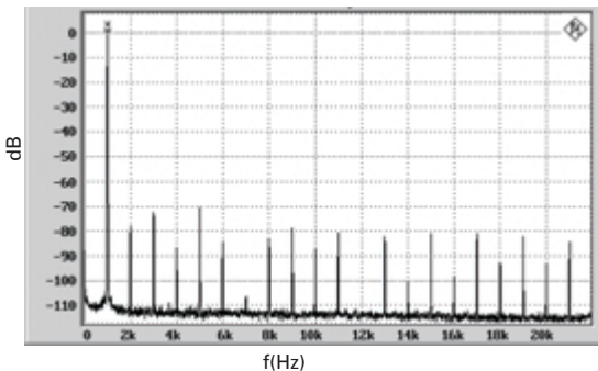
FFT of distortion and noise floor at 1W (4 load)
