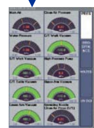
Condition monitor screen
