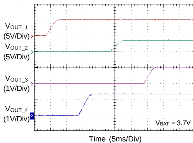
Power On Sequence 5
