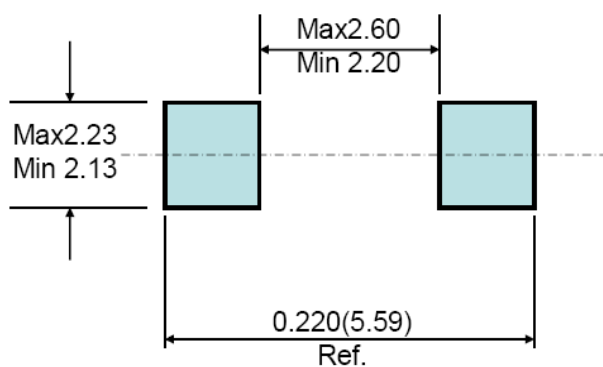
Mounting Pad Layout ---SMB
