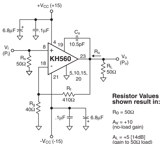
Figure 1: Test Circuit
