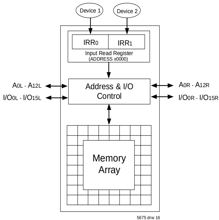
Figure 3. Input Read Register
