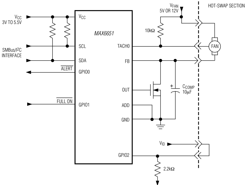
Figure 13. Hot-Swap Application
