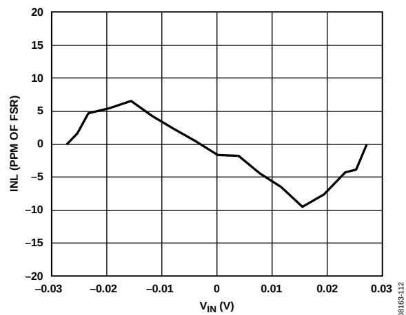
Figure 12. INL (Gain = 128)
