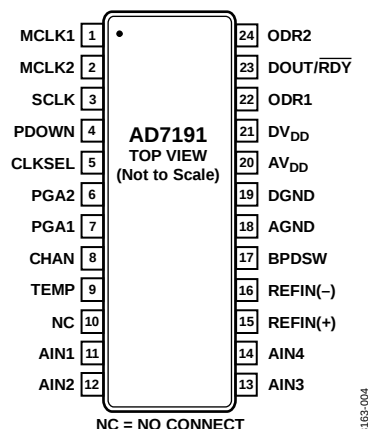
Figure 4. Pin Configuration
