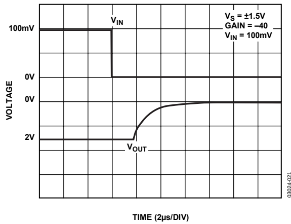
Figure 21. Saturation Recovery
