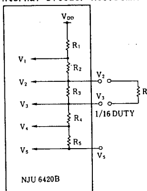
Internal Bleeder Resistance
