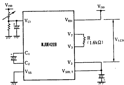
(b) 1/5 Bias (1/16 Duty) (Internal Voltage Doubler Using Example)
