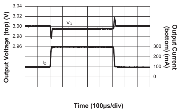
Load Transient Response LDO1 I_{OUT1} = 100mA \text{ to } 300mA ; V_{BAT} = 3.6V ; V_{OUT1} = 3V
