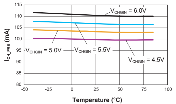
Preconditioning Charge Current vs. Temperature ( V_{BAT} = 2.5V , R_{SET} = 1.24k\Omega )
