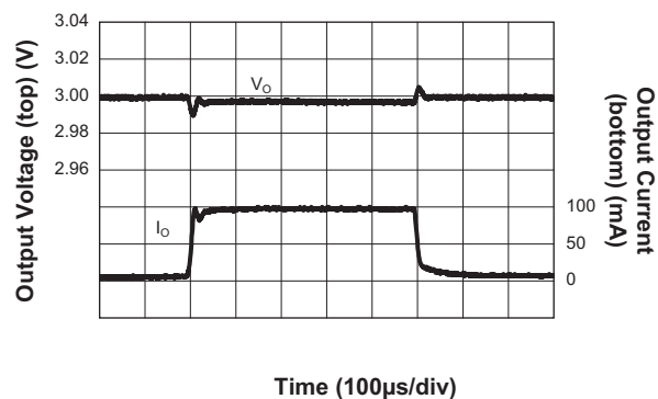
Load Transient Response LDO1 I_{OUT1} = 10mA \text{ to } 100mA ; V_{BAT} = 3.6V ; V_{OUT1} = 3V
