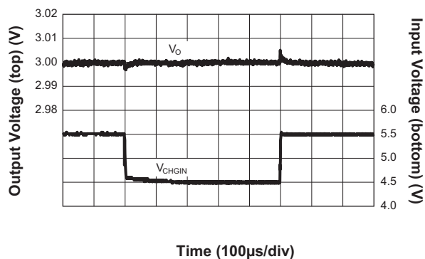
Line Transient Response LDO1 V_{CHGIN} = 4.5V \text{ to } 5.5V ; I_{OUT} = 300mA ; V_{OUT} = 3V
