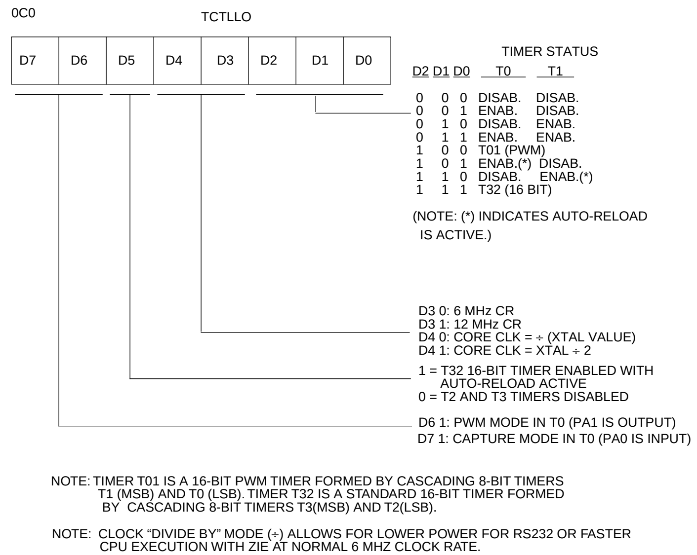
Figure 25. TCTLLO Register
