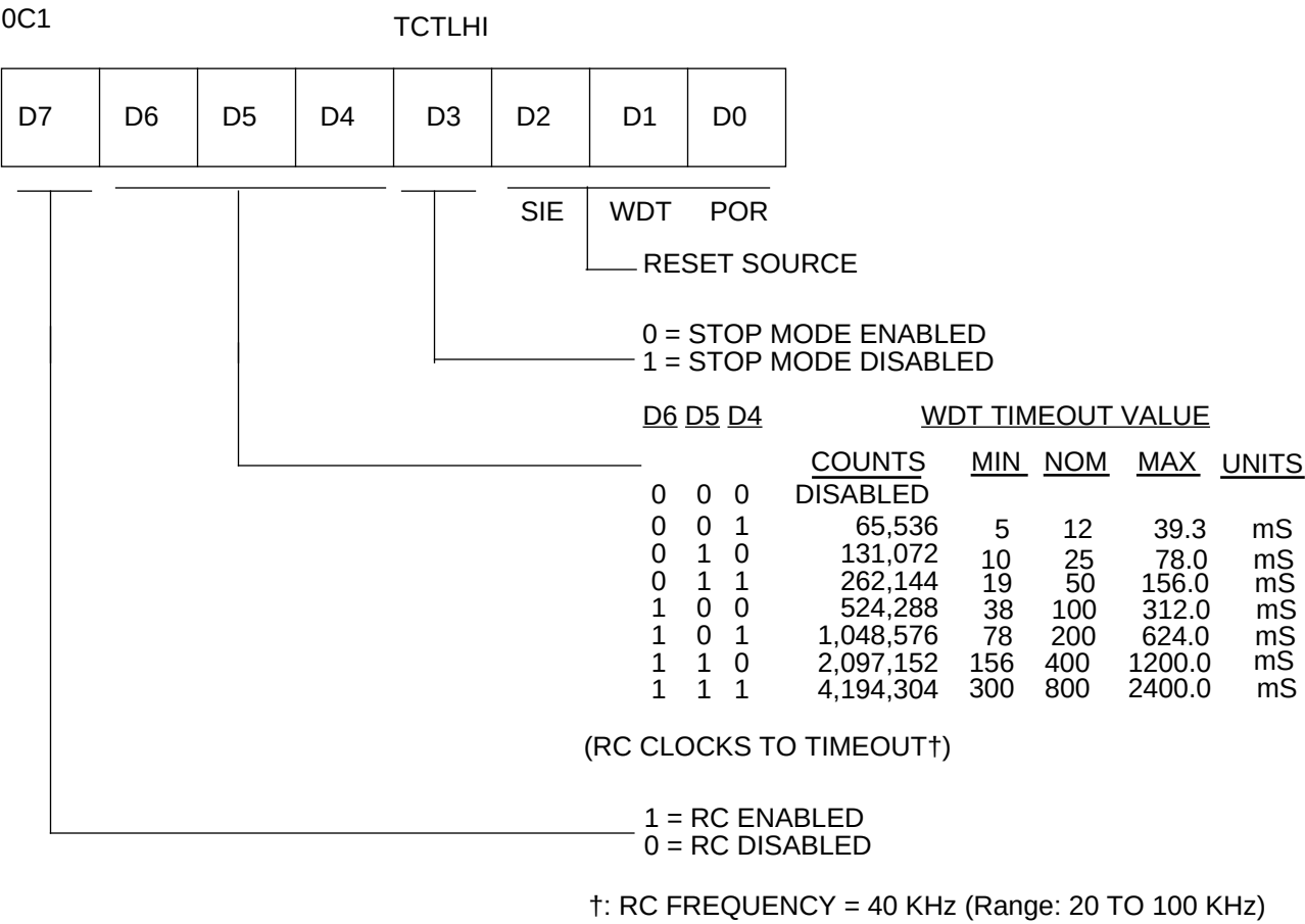
Figure 24. TCTLHI Register
