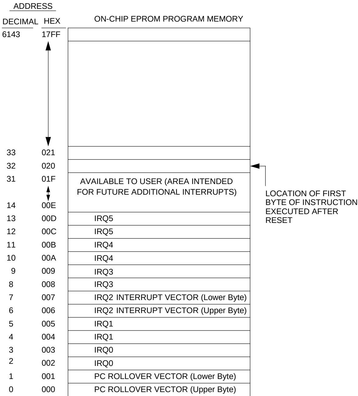
Figure 11. Z8E520 Program Memory Map
