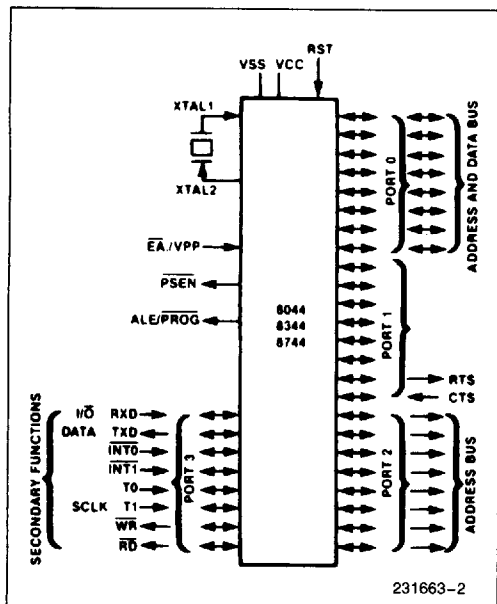
Figure 2. Logic Symbol
