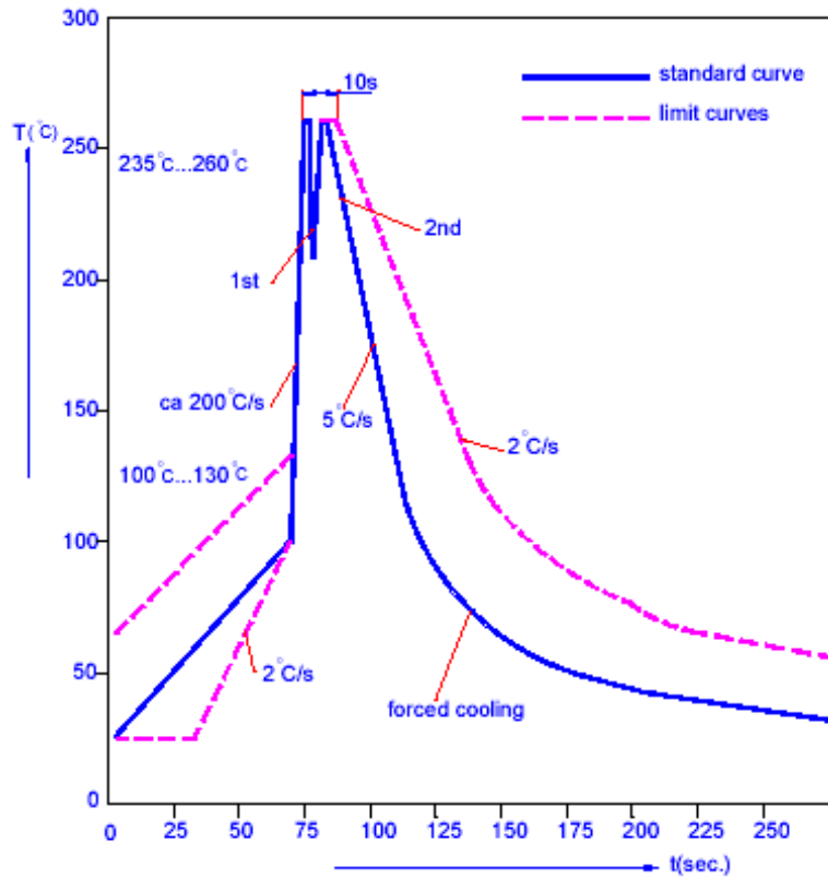
Fig. 7 Recommended TTW Soldering Profile.
