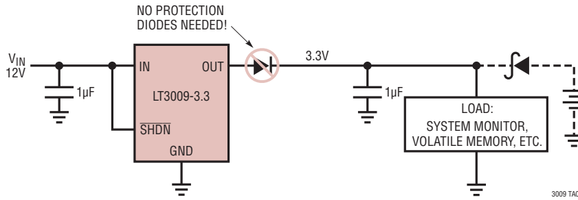
Keep-Alive Power Supply
