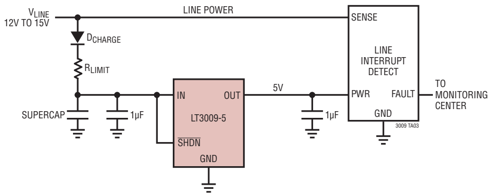
Last-Gasp Circuit
