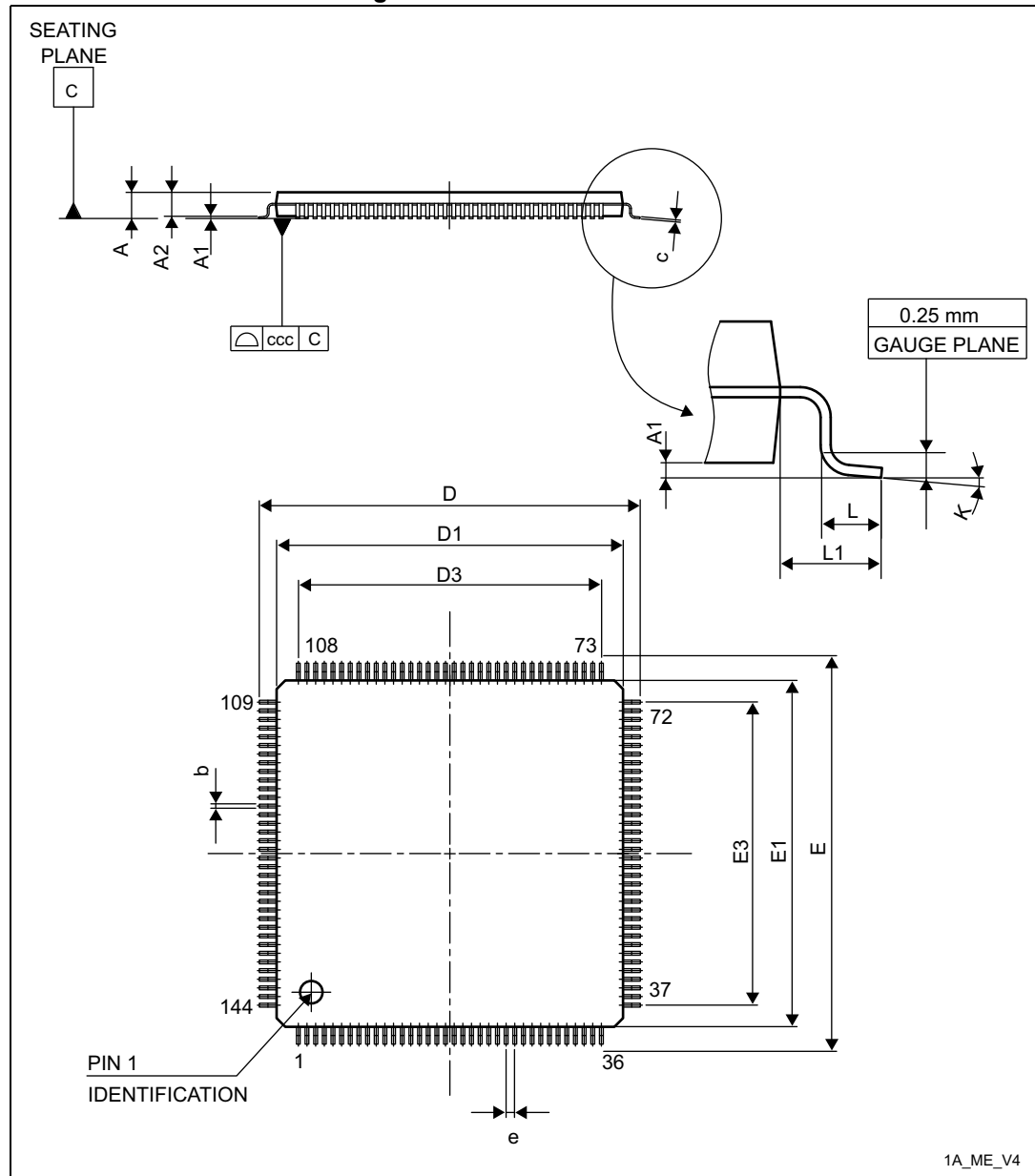
Figure 83. LQFP144 - Outline
