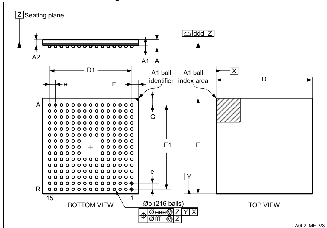
Figure 98. TFBGA216 - Outline
