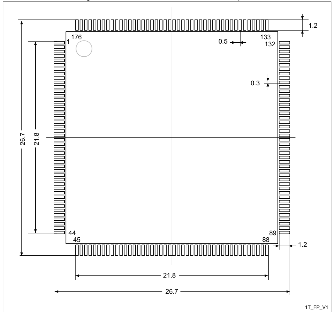
Figure 91. LQFP176 - Recommended footprint
