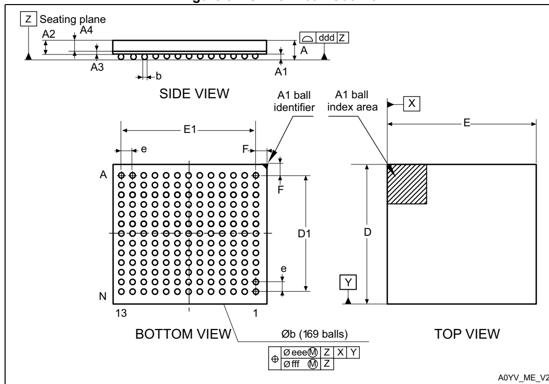
Figure 87. UFBGA169 - Outline
