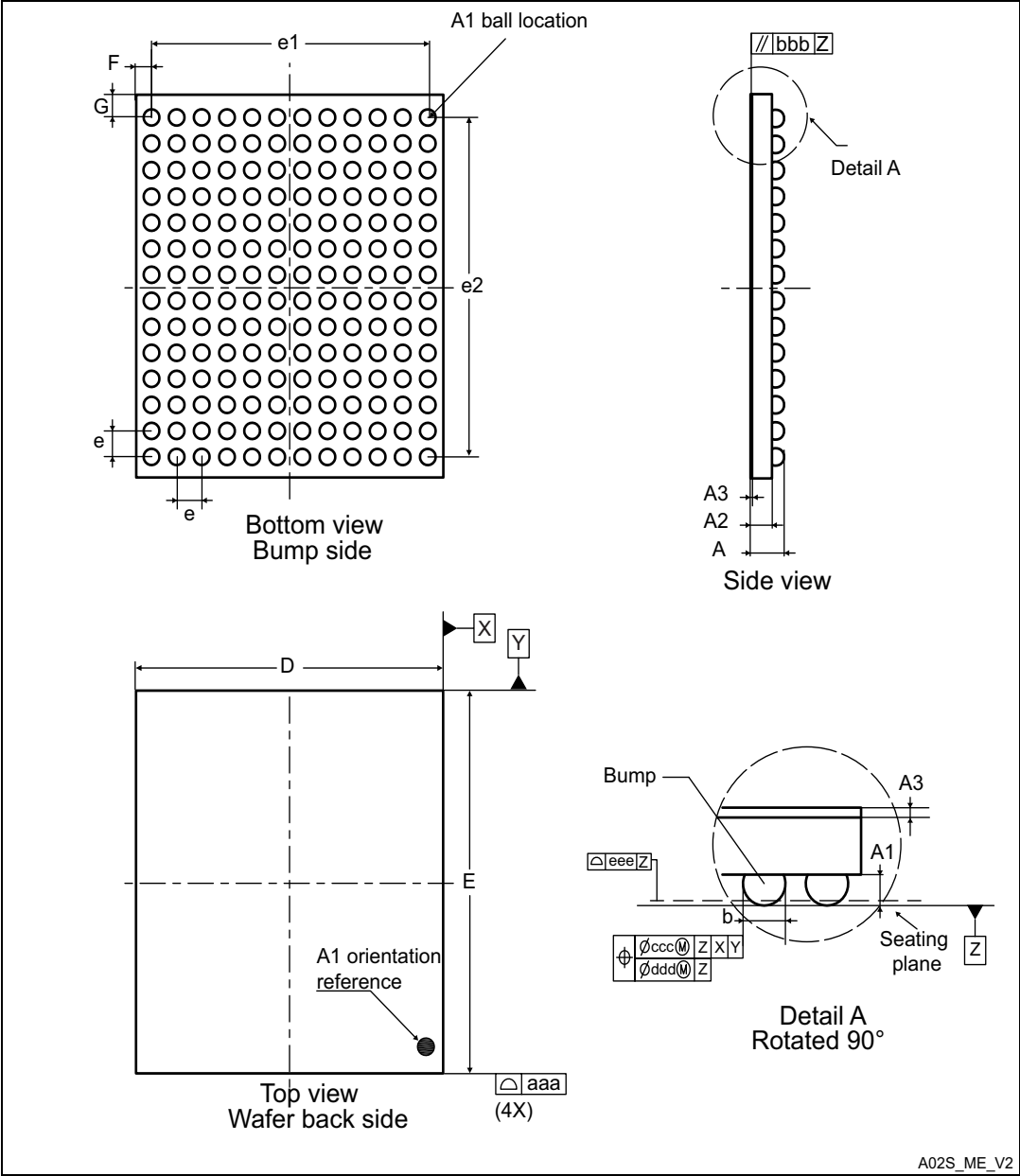
Figure 86. WLCSP168 - Outline
