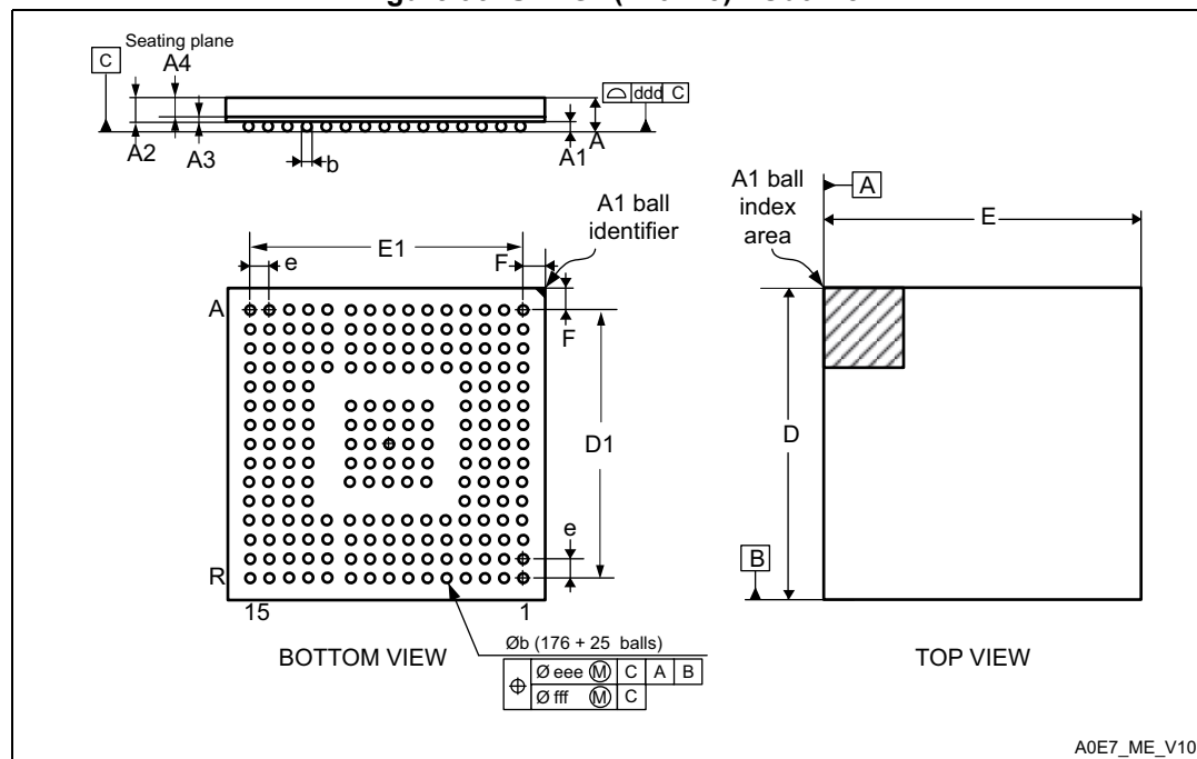
Figure 93. UFBGA(176+25) - Outline
