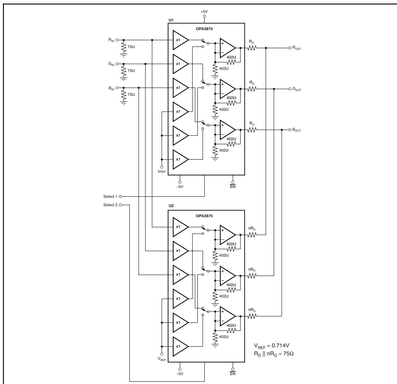
Figure 28. Logo Inserter
