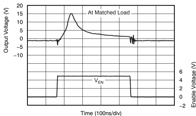
DISABLE/ENABLE SWITCHING GLITCH
