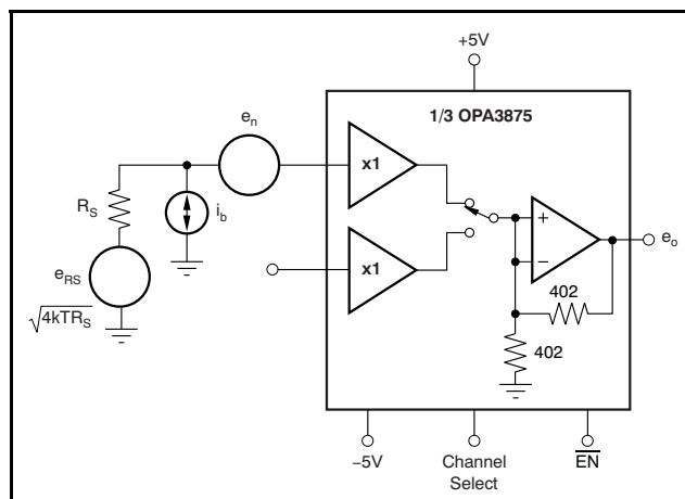
Figure 30. Noise Model
