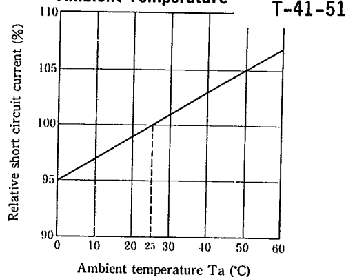
Fig. 2 Relative Short Circuit Current vs. Ambient Temperature
