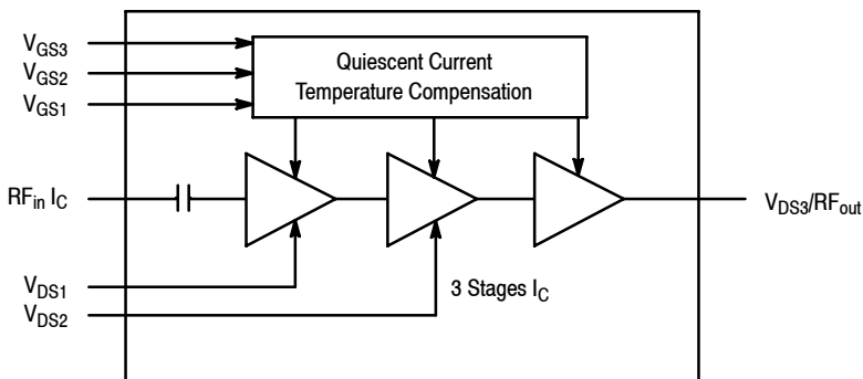
Figure 1. Block Diagram
