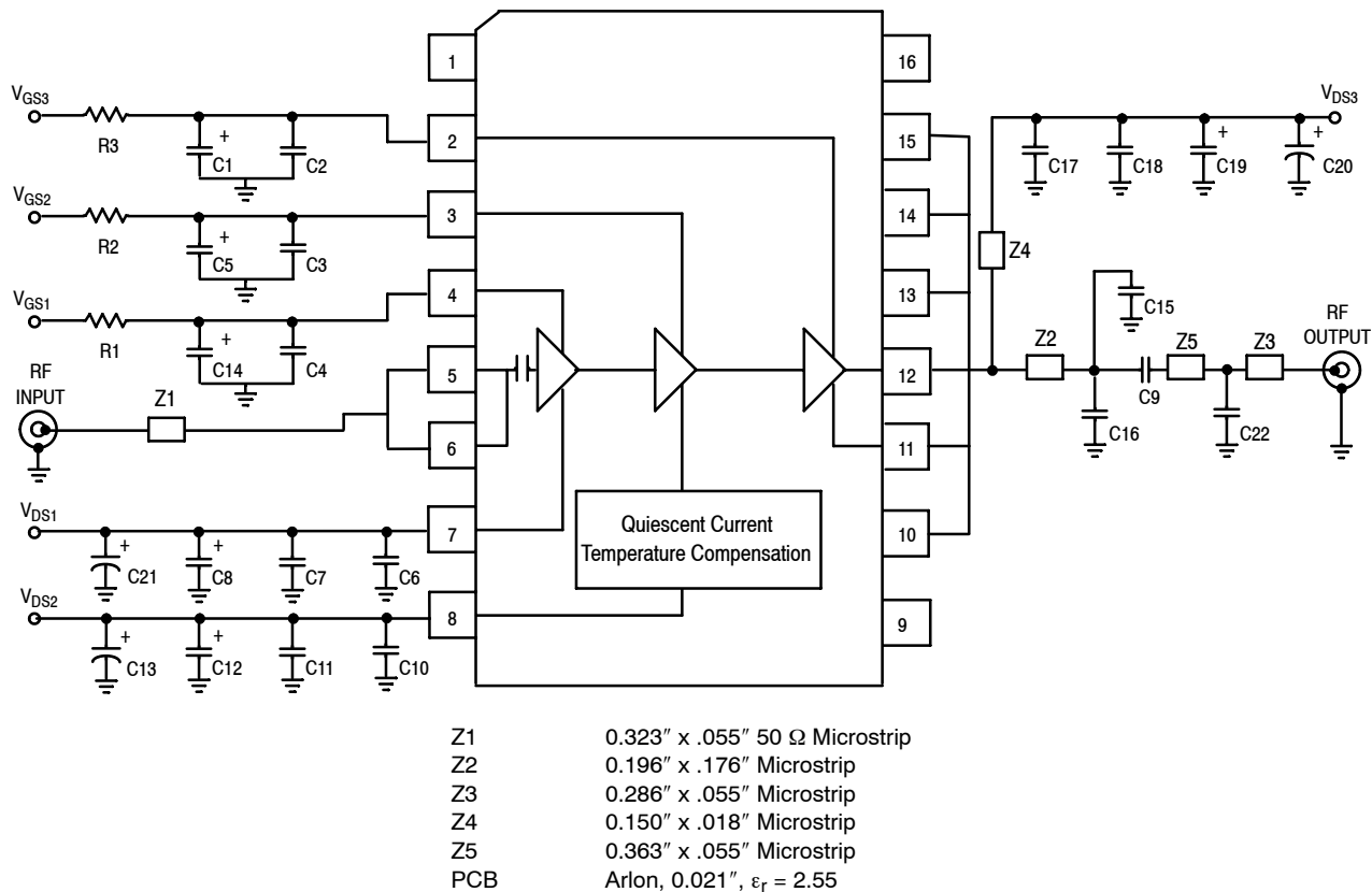
Figure 3. MHVIC2114NR2 Test Circuit Schematic
