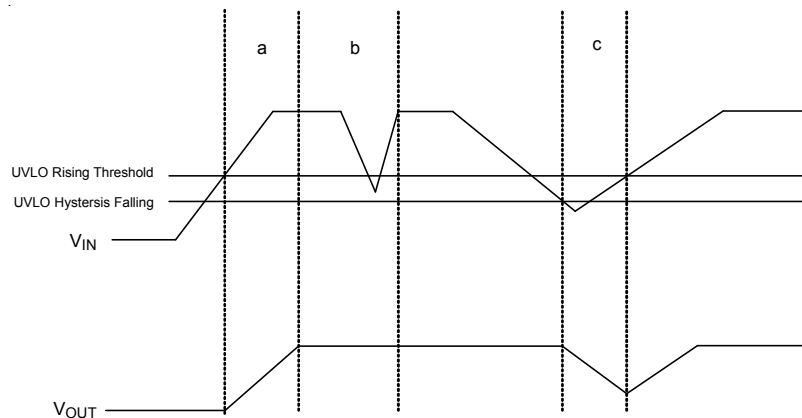
Figure 5. Under Voltage Lockout Trimming Conditions and Output Variation
