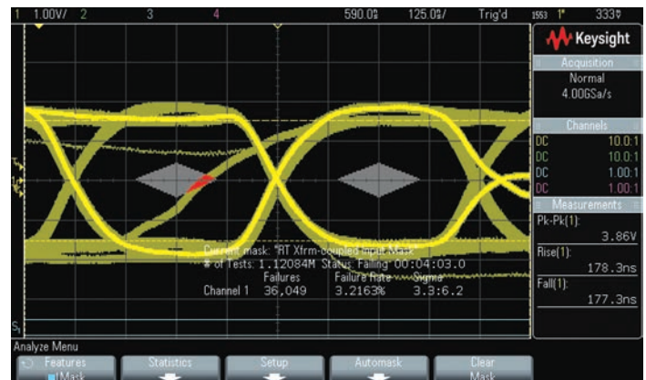
Figure 8. MIL-STD 1553 BC to RT xfrm-coupled input mask test reveals a shifted bit that violates the pass/fail mask.
