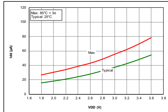
FIGURE 26-2: I_{DD} , EC Oscillator, 500 kHz, PIC16LF1566/67 Only
