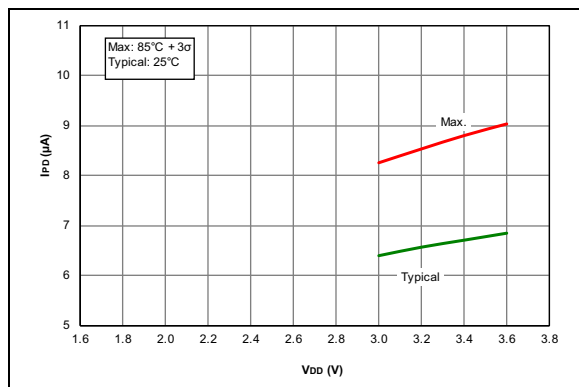
FIGURE 26-13: IPD , Brown-out Reset (BOR), BORV = 1 , PIC16LF1566/67 Only
