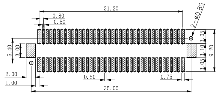
RECOMMENDED PCB LAYOUT TOLERANCE: ±0.05mm
