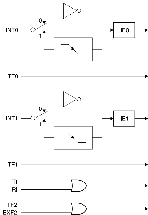
Figure 6. Interrupt Sources
