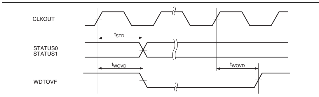
Figure 33.6 Pin Drive Timing in Standby
