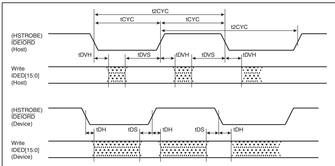
Figure 33.49 Ultra-DMA Data Out-burst
