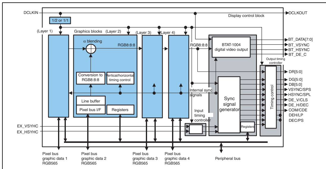
Figure 24.1 Block Diagram of VDC2
