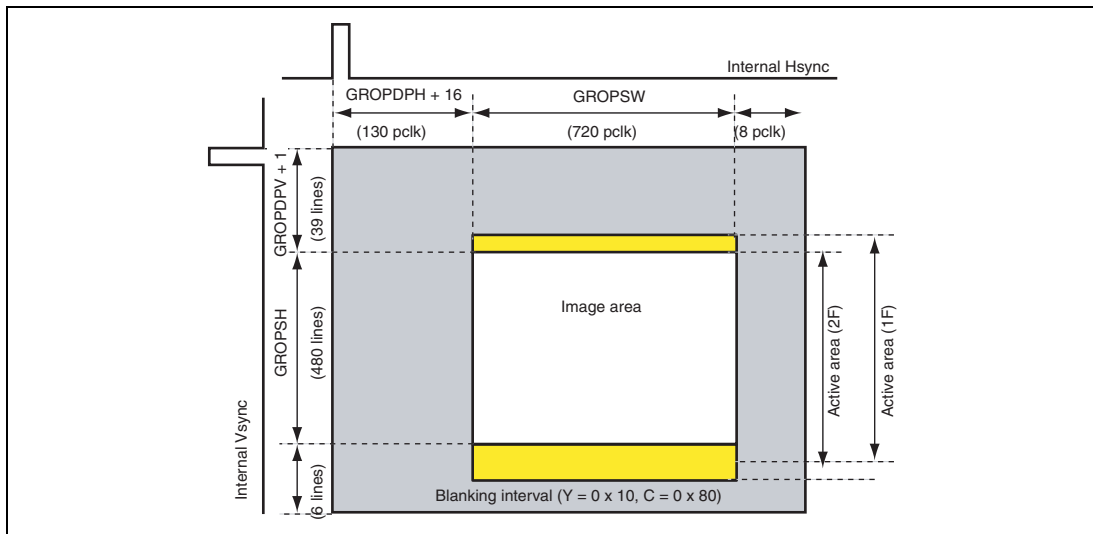
Figure 24.15 T-1004 Video Output Position
