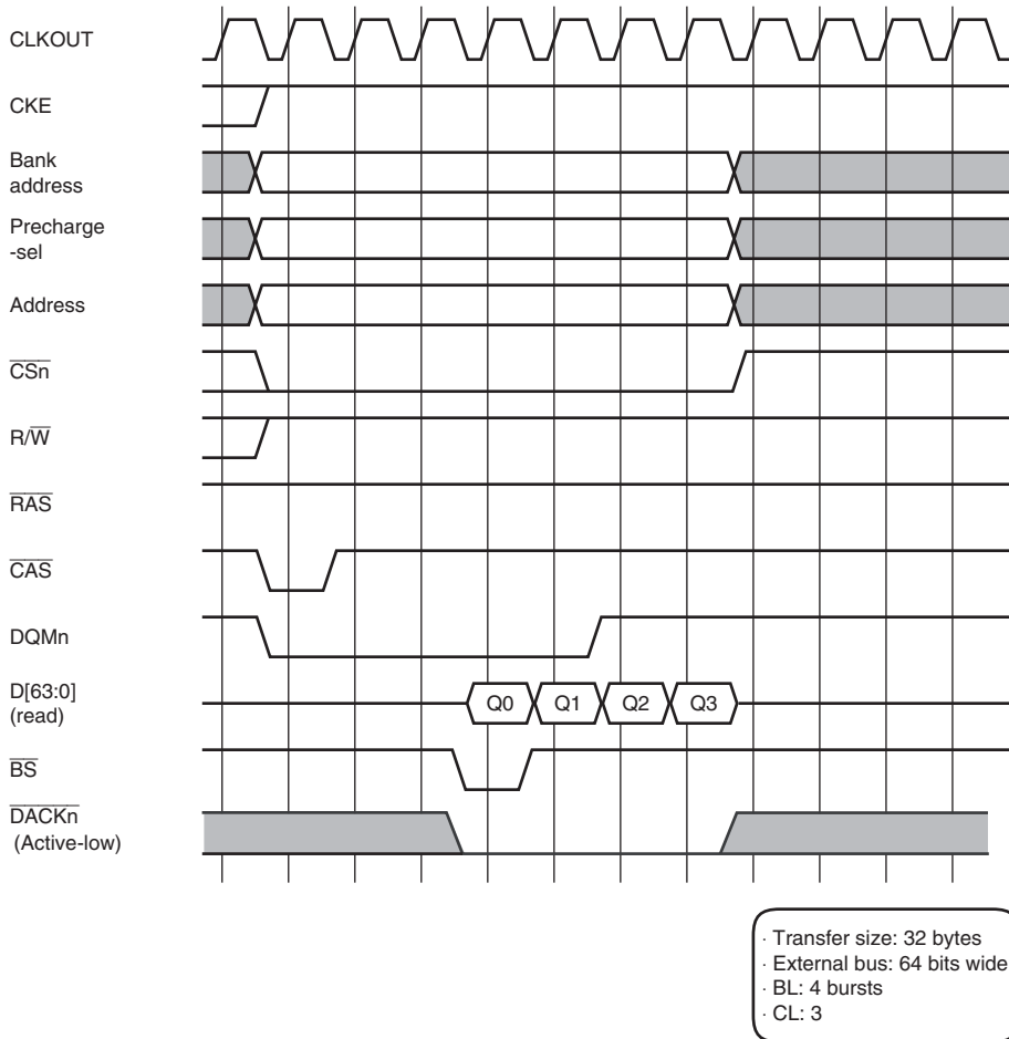
Figure 11.16 Basic SDRAM Interface Timing (5) Burst Read Timing (Bank Open Mode; Same Row Address Accessed)
