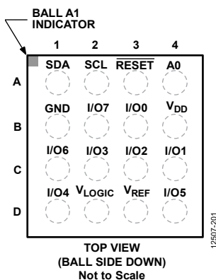
Figure 5. 16-Ball WLCSP Pin Configuration
