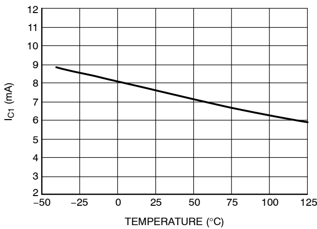
Figure 7. Internal Startup Current Source at V CC = 10 V versus Temperature
