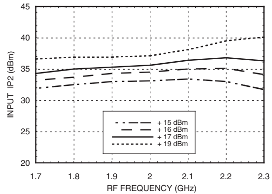
Input IP2 vs. LO Drive @ LO = +17 dBm
