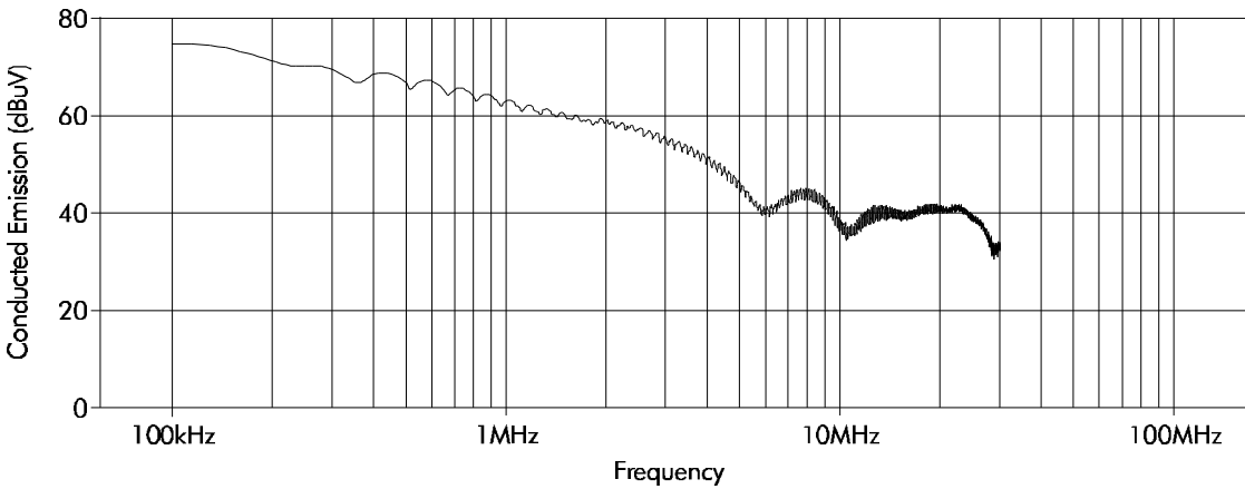
NME48 series spectrum analysis RBW 100kHz
