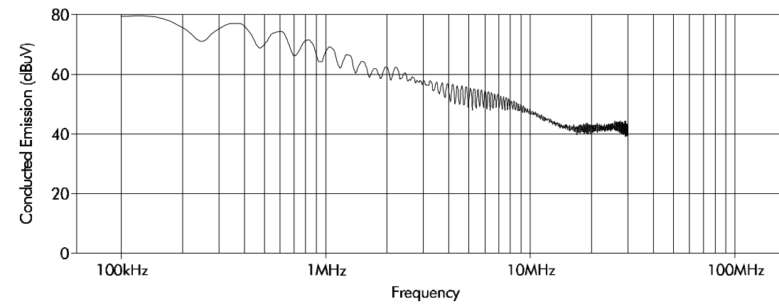
NME48 series spectrum analysis RBW 100kHz
