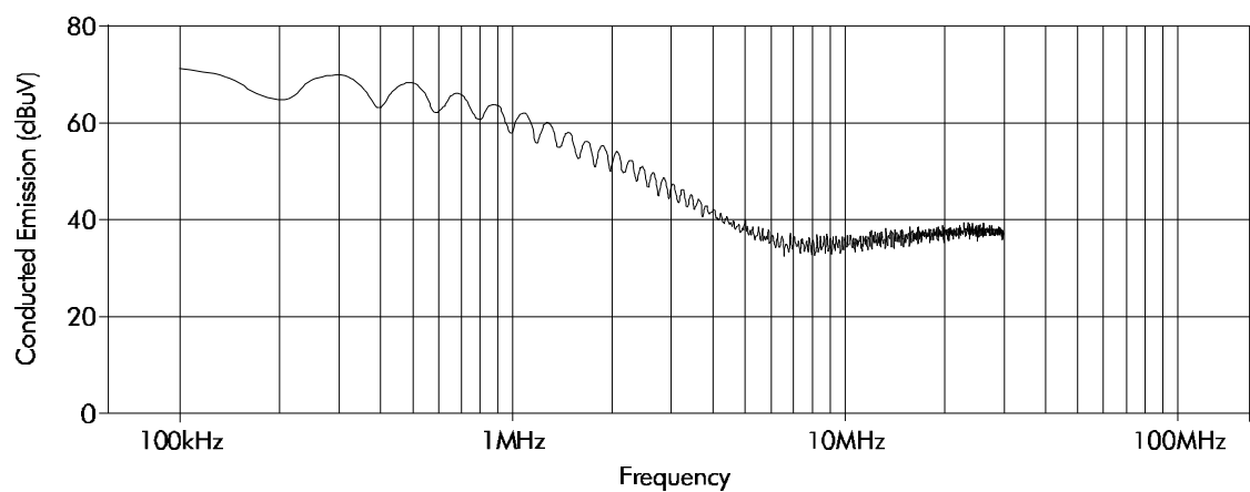
NME12 series spectrum analysis RBW 100kHz
