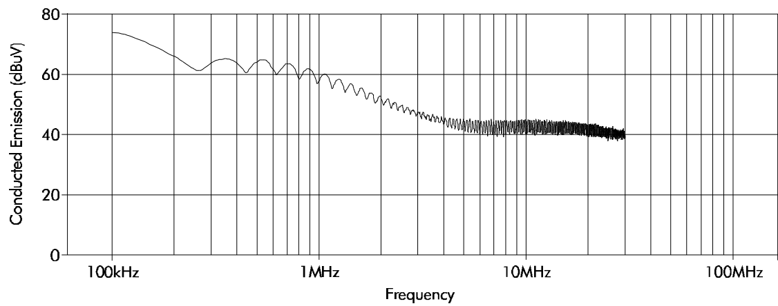
NME05 series spectrum analysis RBW 100kHz
