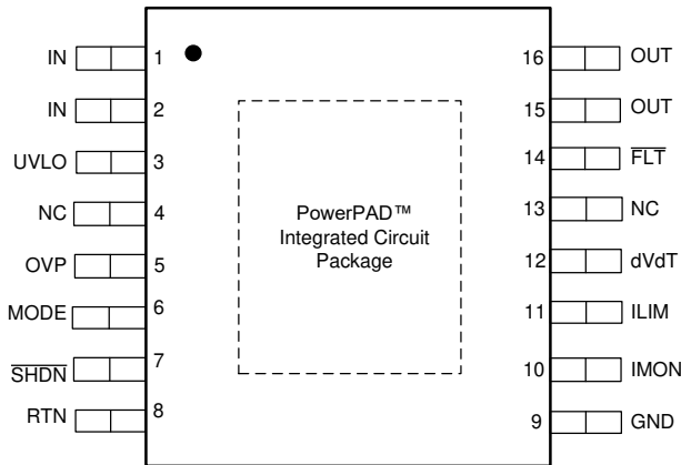
Figure 6-1. PWP Package 16-Pin HTSSOP Top View
