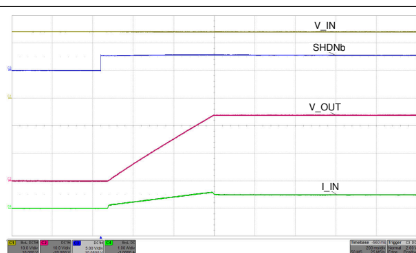
Figure 10-10. Start-Up With Shutdown Pin—48-Ω Load
