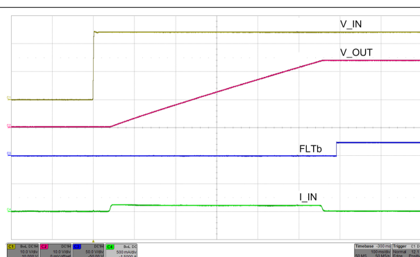
Figure 10-8. Start-Up With VIN—No Load
