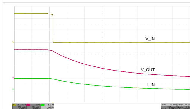
Figure 10-9. Power Fail With 24-Ω Load—Supports 1-A Load for 10-ms Power Fail
