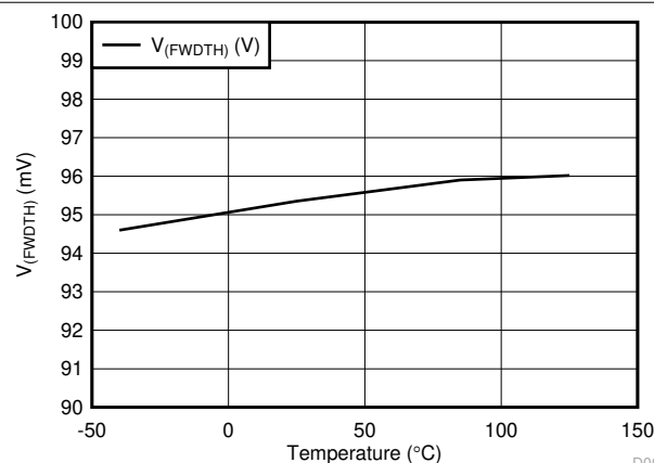
Figure 7-5. V_{(FWDTH)} vs Temperature
