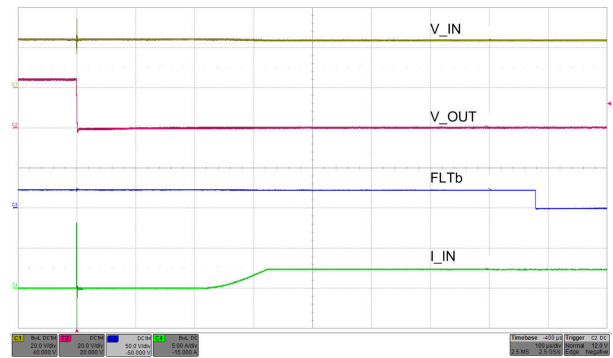
Figure 9-13. Zoomed at the Instance of Output Short
