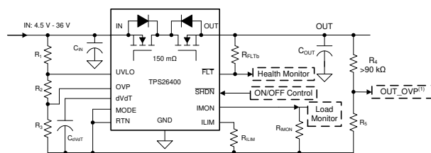
Simplified Schematic
