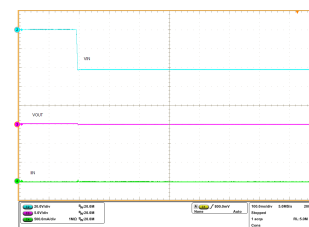
Reverse Polarity Protection with -42\text{ V} Input
