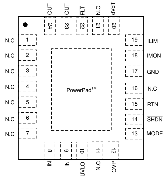
Figure 6-2. RHF Package 24-Pin VQFN Top View
