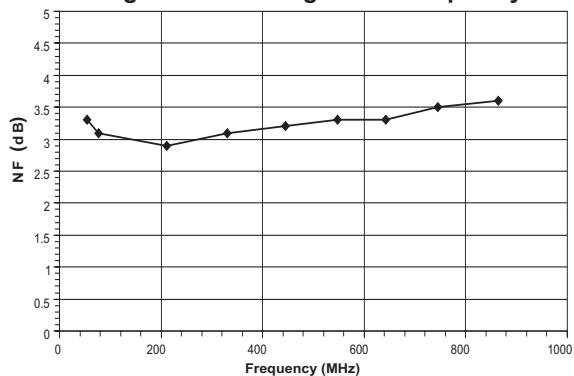
Figure 8: Noise Figure vs. Frequency
