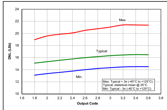
FIGURE 38-116: DAC INL Error, V_{DD} = 3.0V , PIC16LF1777/8/9 Only.
