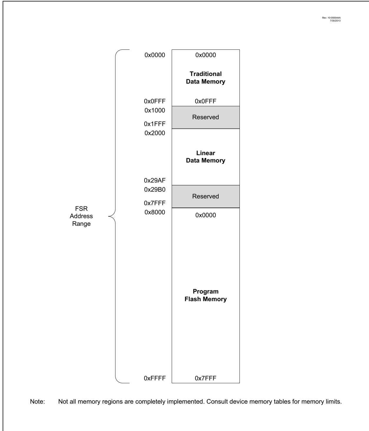
FIGURE 3-9: INDIRECT ADDRESSING
