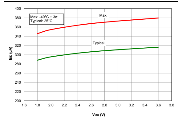
FIGURE 38-50: I_{PD} , Comparator, NP Mode ( V_{REGPM} = 0 ), PIC16LF1777/8/9 Only.
