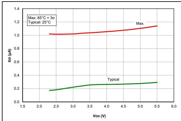
FIGURE 38-49: I_{PD} , ADC Non-Converting, PIC16F1777/8/9 Only.
