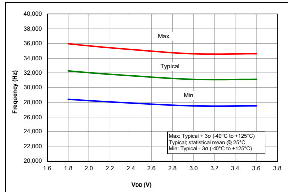
FIGURE 38-58: LFINTOSC Frequency, PIC16LF1777/8/9 Only.
