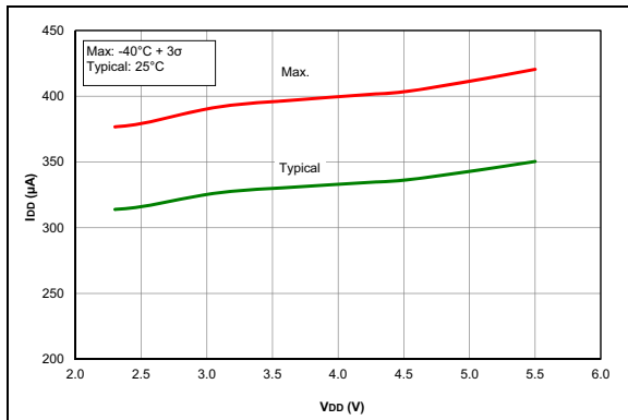
FIGURE 38-51: I_{PD} , Comparator, NP Mode ( V_{REGPM} = 0 ), PIC16F1777/8/9 Only.
