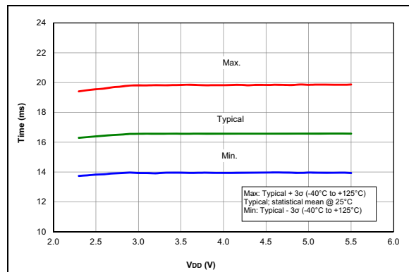
FIGURE 38-60: WDT Time-Out Period, PIC16F1777/8/9 Only.
