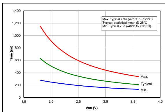
FIGURE 38-110: Comparator Output Filter Delay Time Over Temp., NP Mode, Typical Measured Values, PIC16F1777/8/9 Only.
