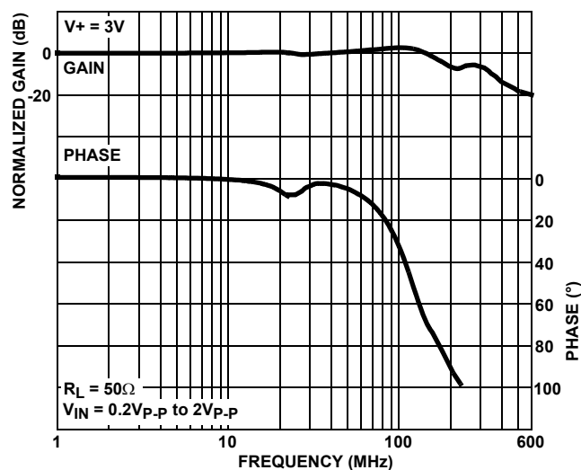
FIGURE 15. FREQUENCY RESPONSE
