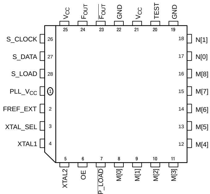
Figure 2. 28–Lead PLCC (Top View)
