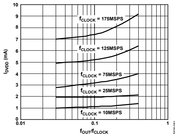
Figure 82. I_{DVDD} vs. f_{OUT}/f_{CLOCK} Ratio at DVDD = 3.3 V
