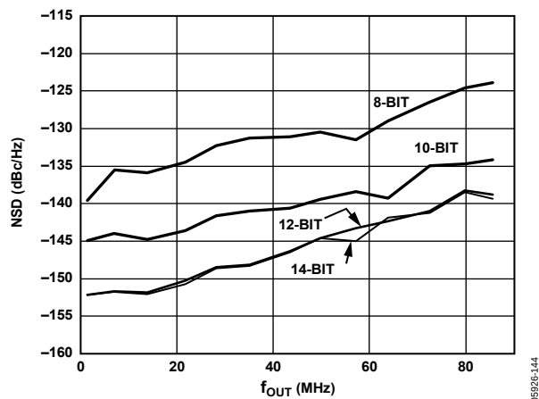
Figure 44. AD9704/AD9705/AD9706/AD9707 NSD vs. f_{OUT} at 0 dBFS, 175 MSPS
