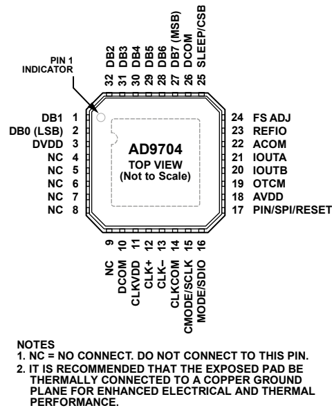
Figure 6. AD9704 Pin Configuration
