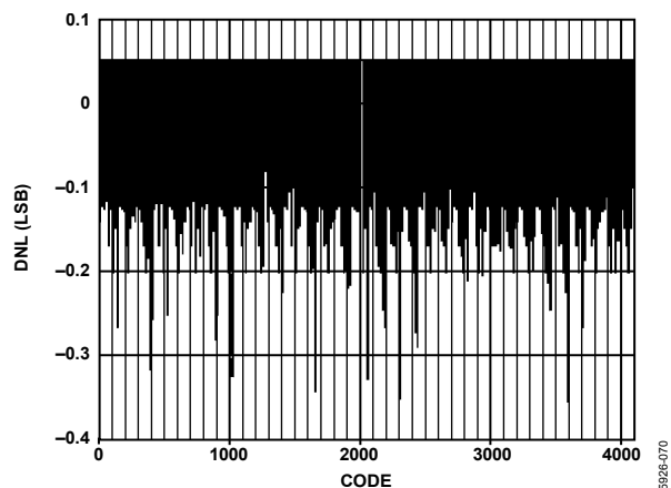
Figure 63. AD9706 Typical Uncalibrated DNL
