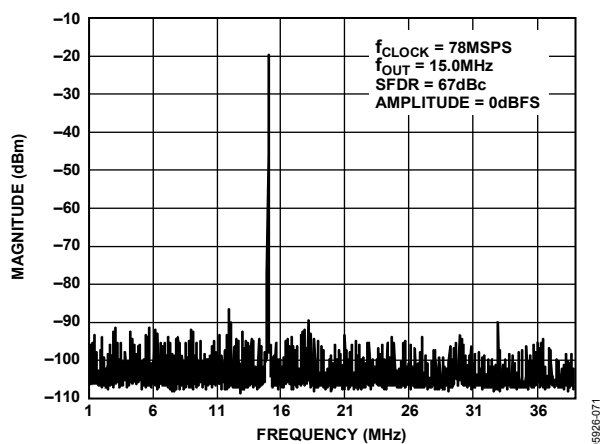
Figure 64. AD9704 Single-Tone SFDR
