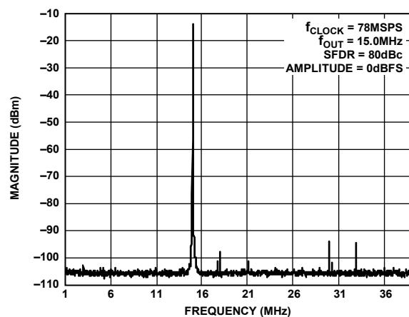
Figure 24. Single-Tone SFDR
