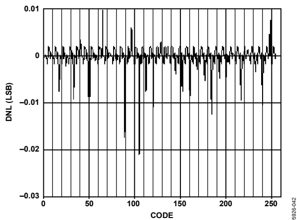
Figure 46. AD9704 Typical Uncalibrated DNL
