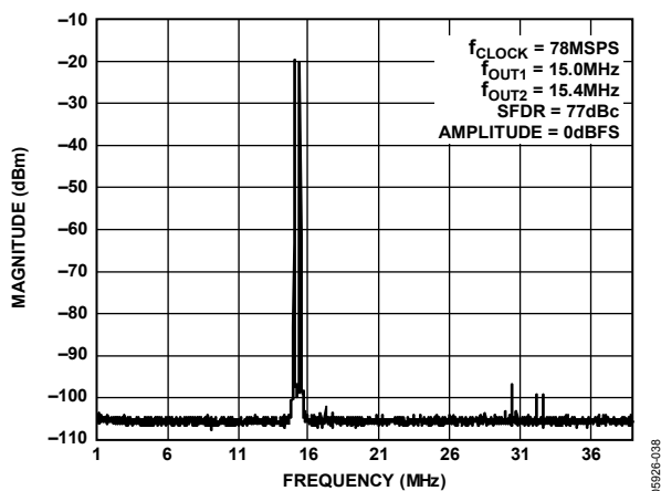
Figure 25. Dual-Tone SFDR
