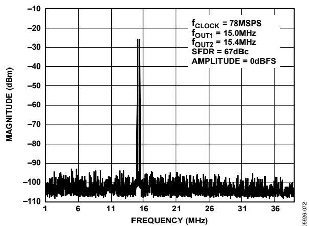
Figure 65. AD9704 Dual-Tone SFDR
