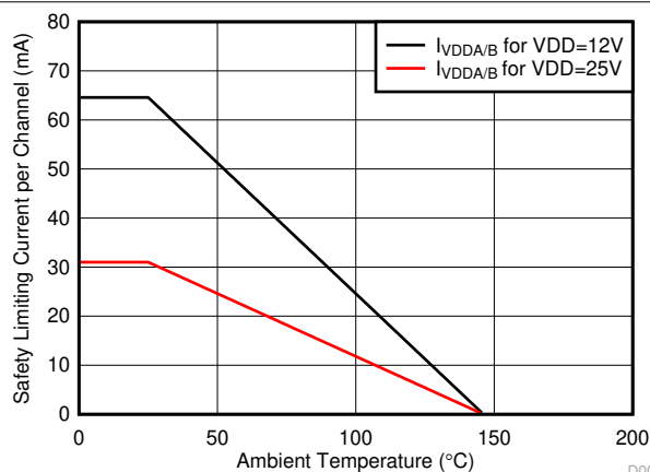
图 6-2. Thermal Derating Curve for Safety-Related Limiting Current (Current in Each Channel with Both Channels Running Simultaneously)
