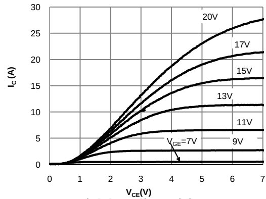
Fig 2: Output Characteristic ( T_j=150^\circ\text{C} )
