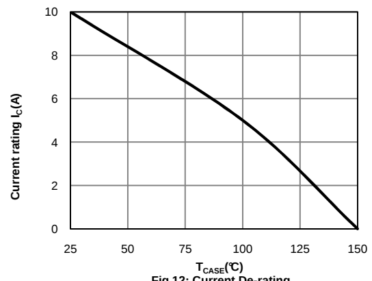
Fig 12: Current De-rating
