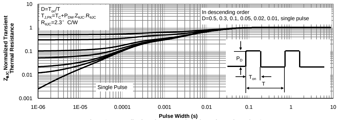
Figure 27: Normalized Maximum Transient Thermal Impedance for IGBT
