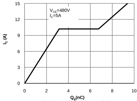
Fig 7: Gate-Charge Characteristics
