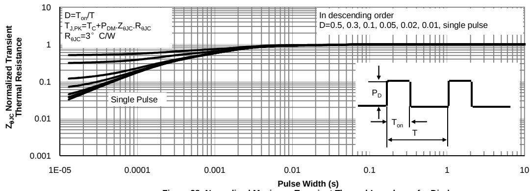
Figure 28: Normalized Maximum Transient Thermal Impedance for Diode
