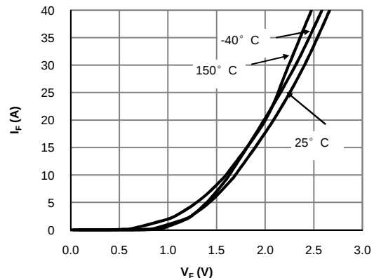
Fig 4: Diode Characteristic
