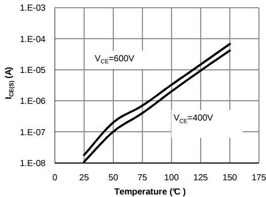
Fig 21: Reverse Leakage Current vs. Junction Temperature
