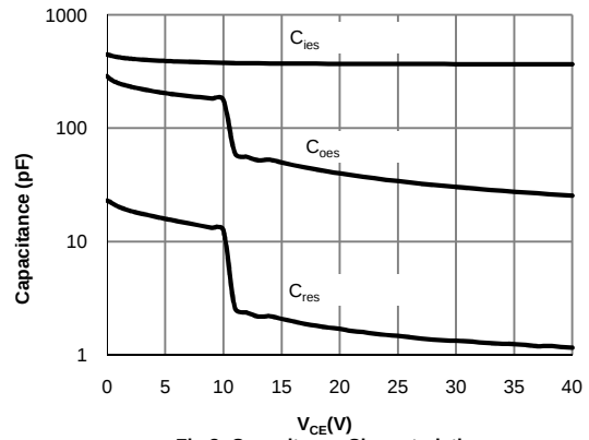
Fig 8: Capacitance Characteristic
