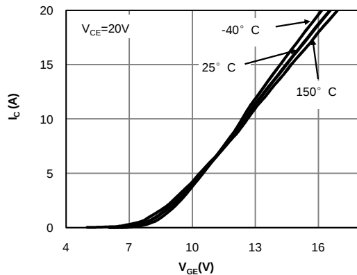
Fig 3: Transfer Characteristic
