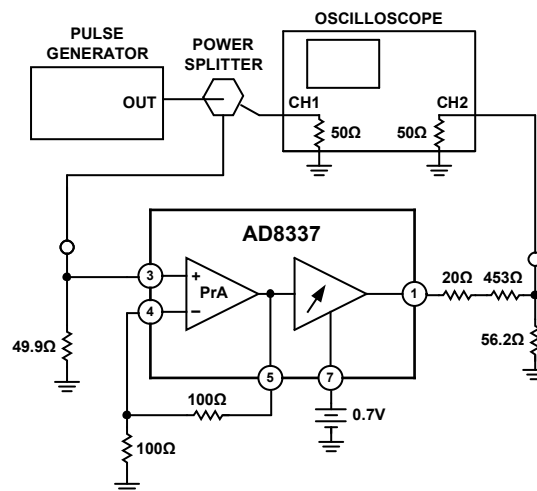
Figure 53. Pulse Response
