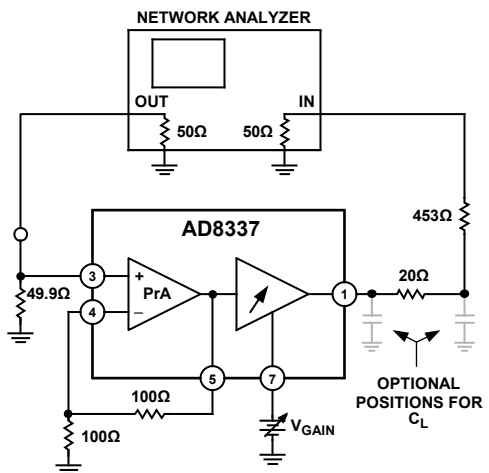
Figure 45. Frequency Response
