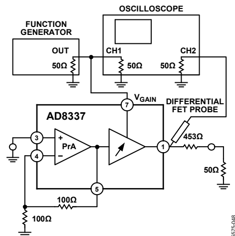
Figure 48. Offset Voltage
