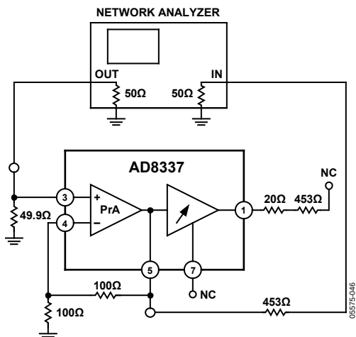
Figure 46. Frequency Response—Preamplifier
