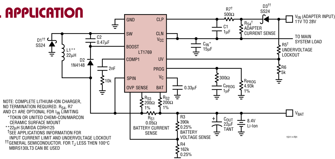
Figure 1. 2A Lithium-Ion Battery Charger
