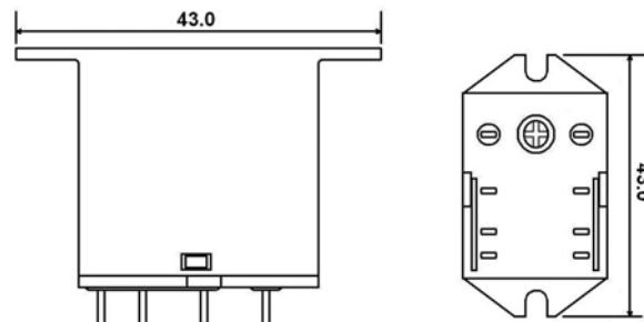
FLANGE MOUNT
