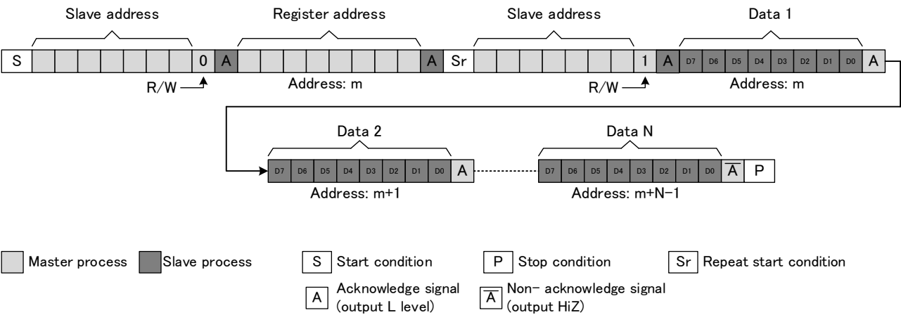
Figure 11.2 read mode format
