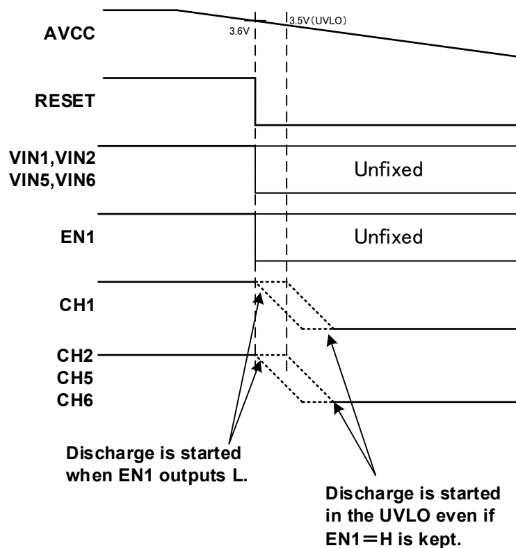
Figure 7.3 Turn off sequence by AVCC voltage drop
