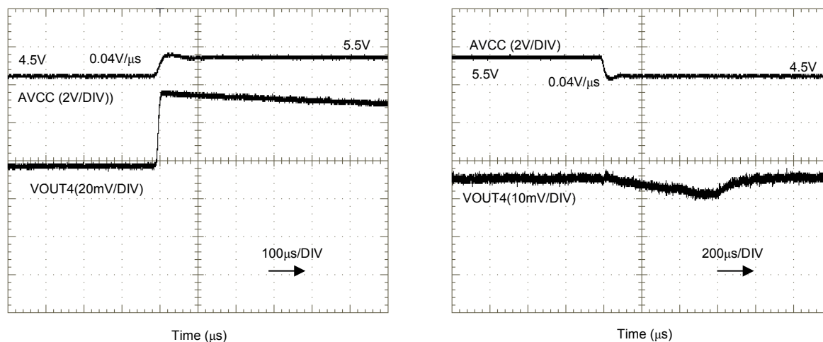
Figure 8.22 Line transient characteristics of CH4 vs AVCC (Reference value)
