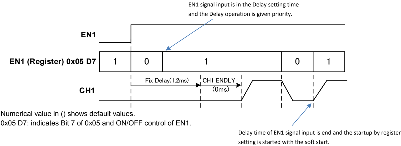
Figure 7.7 Enable control by register setting (0x05)
