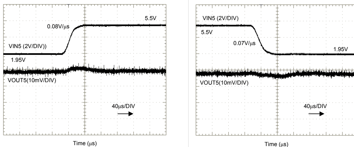
Figure 8.23 Line transient characteristics of CH5 vs VIN5 (Reference value)
