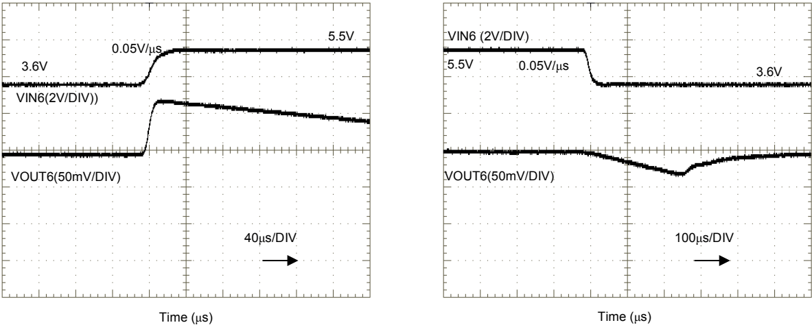
Figure 8.25 Line transient characteristics of CH6 vsVIN6 (Reference value)
