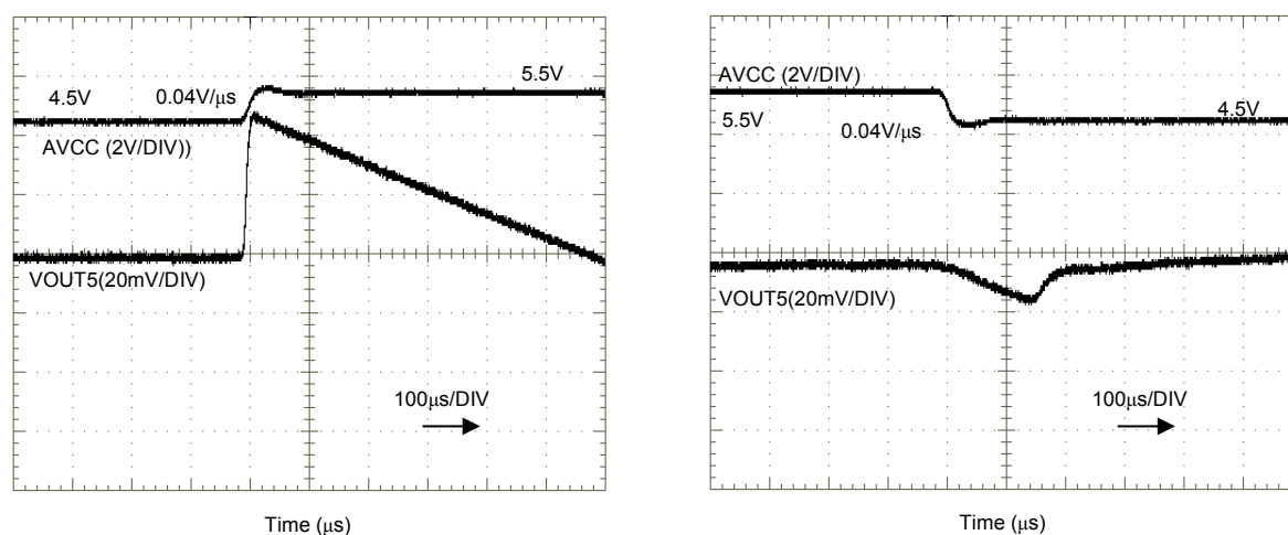
Figure 8.24 Line transient characteristics of CH5 vs AVCC (Reference value)
