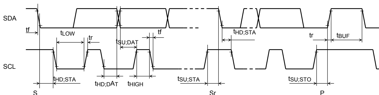
Figure 13.1 AC characteristic
