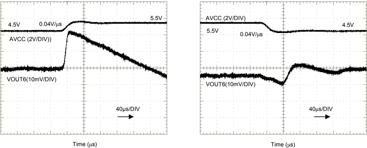
Figure 8.26 Line transient characteristics of CH6 vs AVCC (Reference value)
