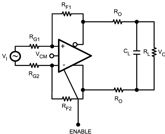
FIGURE 1. Typical Application
