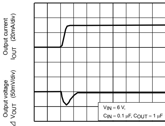
TCR5SB50U ( I_{OUT} = 1\text{m to }30\text{mA} )
