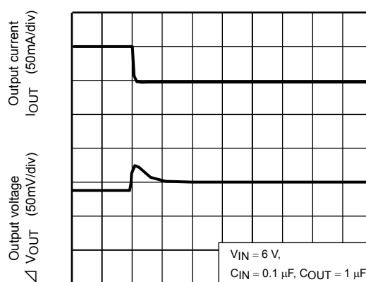
TCR5SB50U ( I_{OUT} = 100\text{m to }50\text{mA} )
