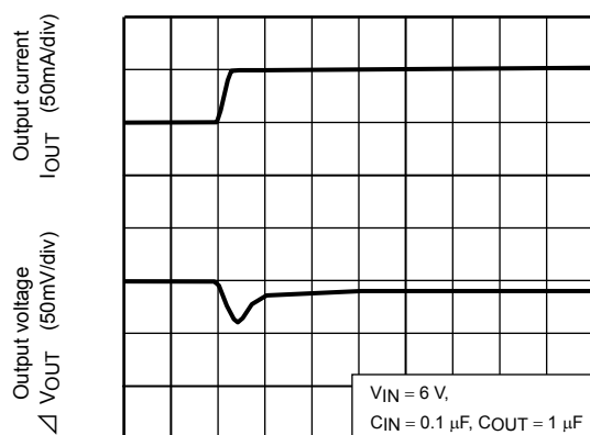
TCR5SB50U ( I_{OUT} = 50\text{m to }100\text{mA} )
