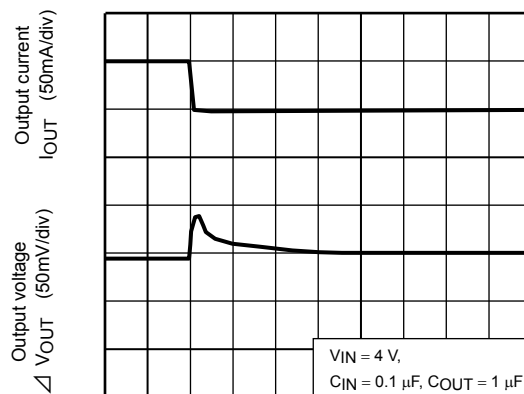
TCR5SB30U ( I_{OUT} = 100\text{m to }50\text{mA} )
