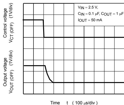
TCR5SB15U (Turn off wave form)
