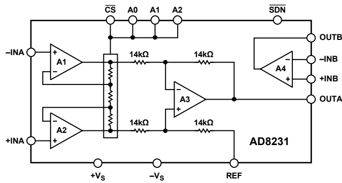
Figure 49. Simplified Schematic
