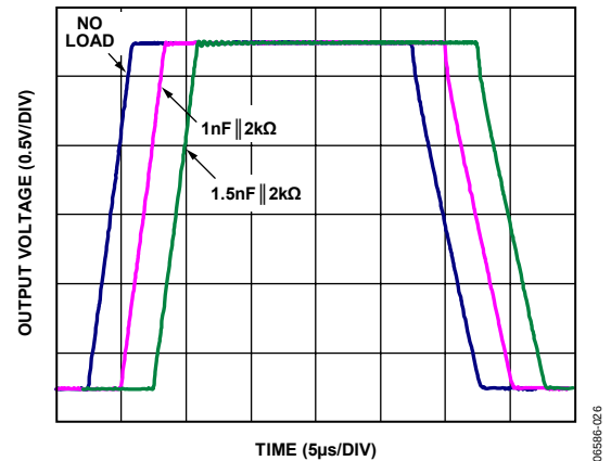
Figure 40. Operational Amplifier Large Signal Transient Response, V_S = 3\text{ V}
