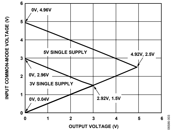
Figure 12. Instrumentation Amplifier Input Common-Mode Range vs. Output Voltage, V_{REF} = 0\text{ V}
