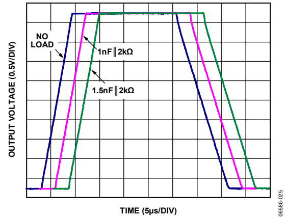
Figure 39. Operational Amplifier Large Signal Transient Response, V_S = 5\text{ V}
