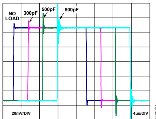
Figure 26. Instrumentation Amplifier Small Signal Pulse Response for Various Capacitive Loads, G = 1
