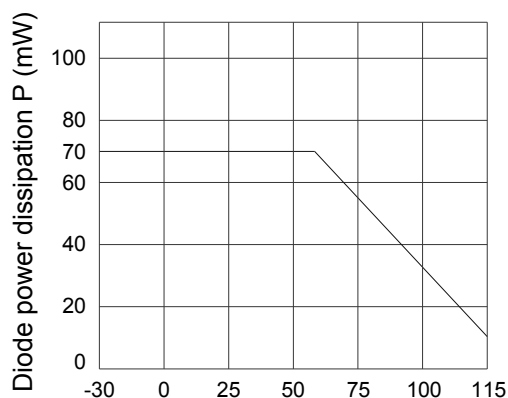
Diode Power Dissipation vs. Ambient Temperature
