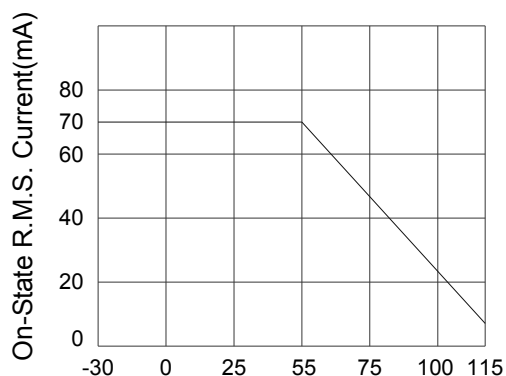
On-State R.M.S. Current vs. Ambient Temperature
