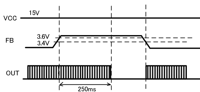
Figure 9, Overload Protection (Self-restart)
