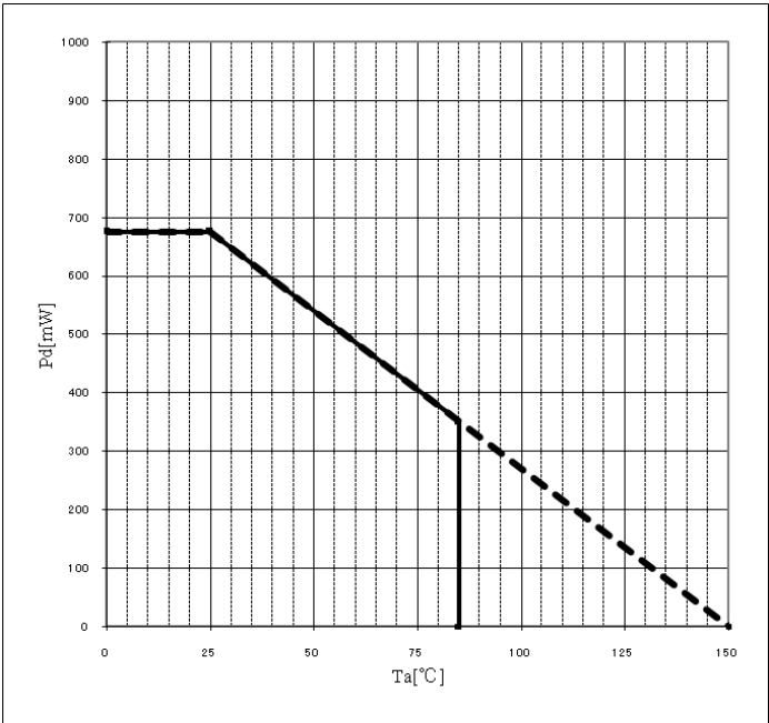
Figure 37, SSOP6 Thermal Reduction Characteristics
