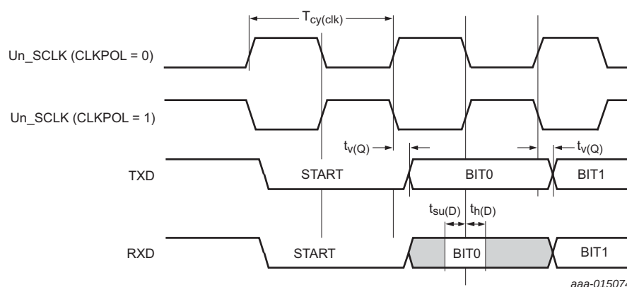
Fig 36. USART timing
