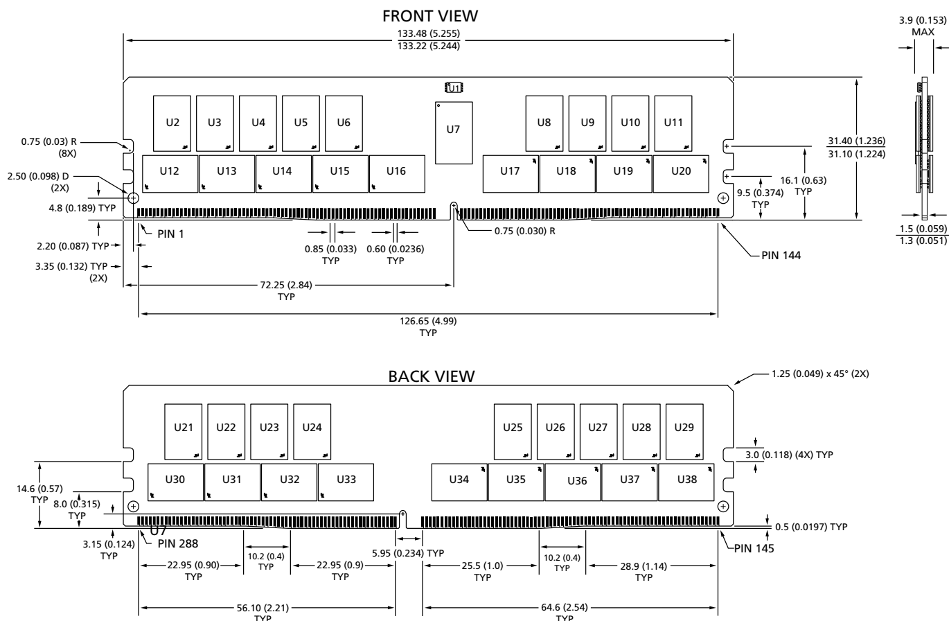
Figure 6: 288-Pin DDR4 RDIMM (R/C-B1, PCB 1971)
